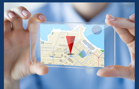
Real-time Validation
